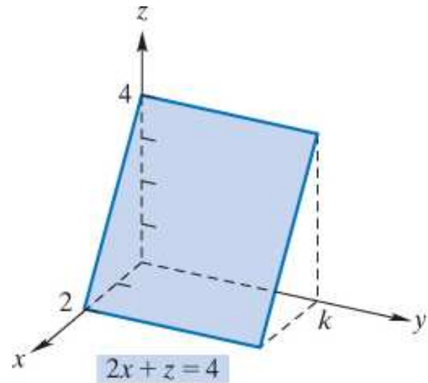
FIGURE 2.41 The plane 2x + z = 4 .
