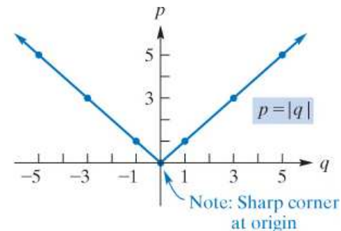
FIGURE 2.14 Graph of p = |q| .
