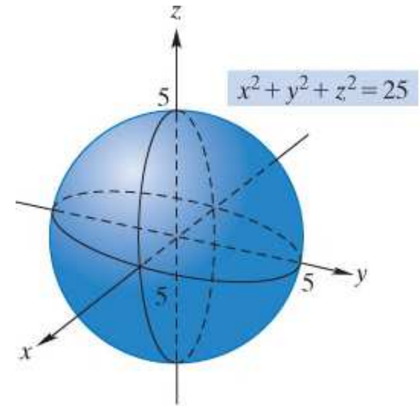
FIGURE 2.43 The surface x^2 + y^2 + z^2 = 25 .
