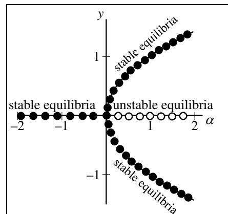
Pitchfork bifurcation at (0, 0)
