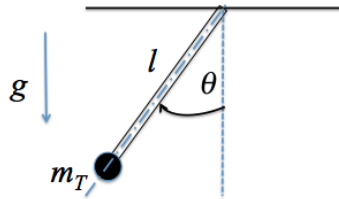
Figure P1.73 A compound pendulum with a tip mass.
