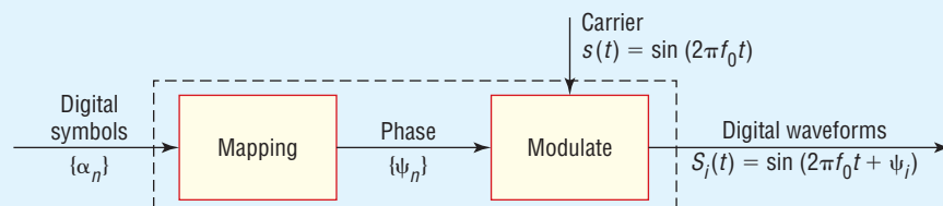
Figure 2 Principle of Phase Modulation
