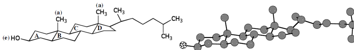
Ball-and-stick model of cholestanol with the H atoms removed for clarity.
