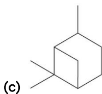
Pinane
