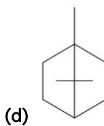
Bornane
