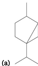
Thujane
