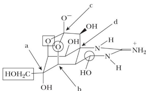
Tetrodotoxin
