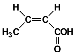
cis -2-Butenoic acid
