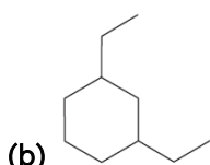
1,3-Diethylcyclohexane
