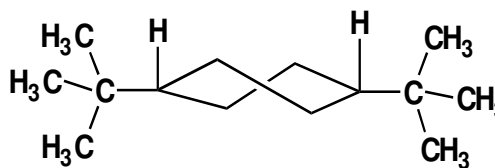
The cis isomer in the twist-boat form
