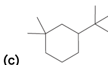
1,1-Dimethyl-3-(1,1-dimethylethyl)-cyclohexane
