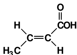
trans -2-Butenoic acid
