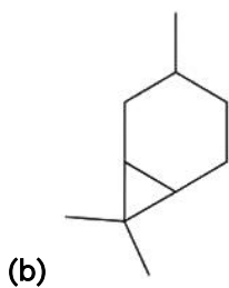
Carane
