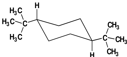
The trans isomer in the chair form
