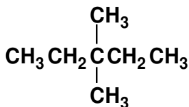
3,3-Dimethylpentane (bp 86.1°C)
