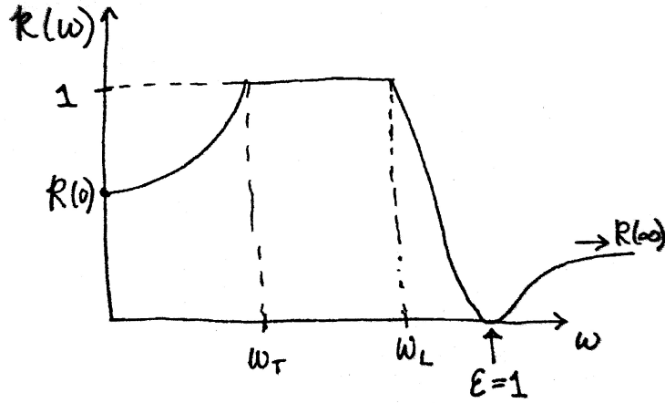
Figure 20: Frequency-dependent reflectivity
