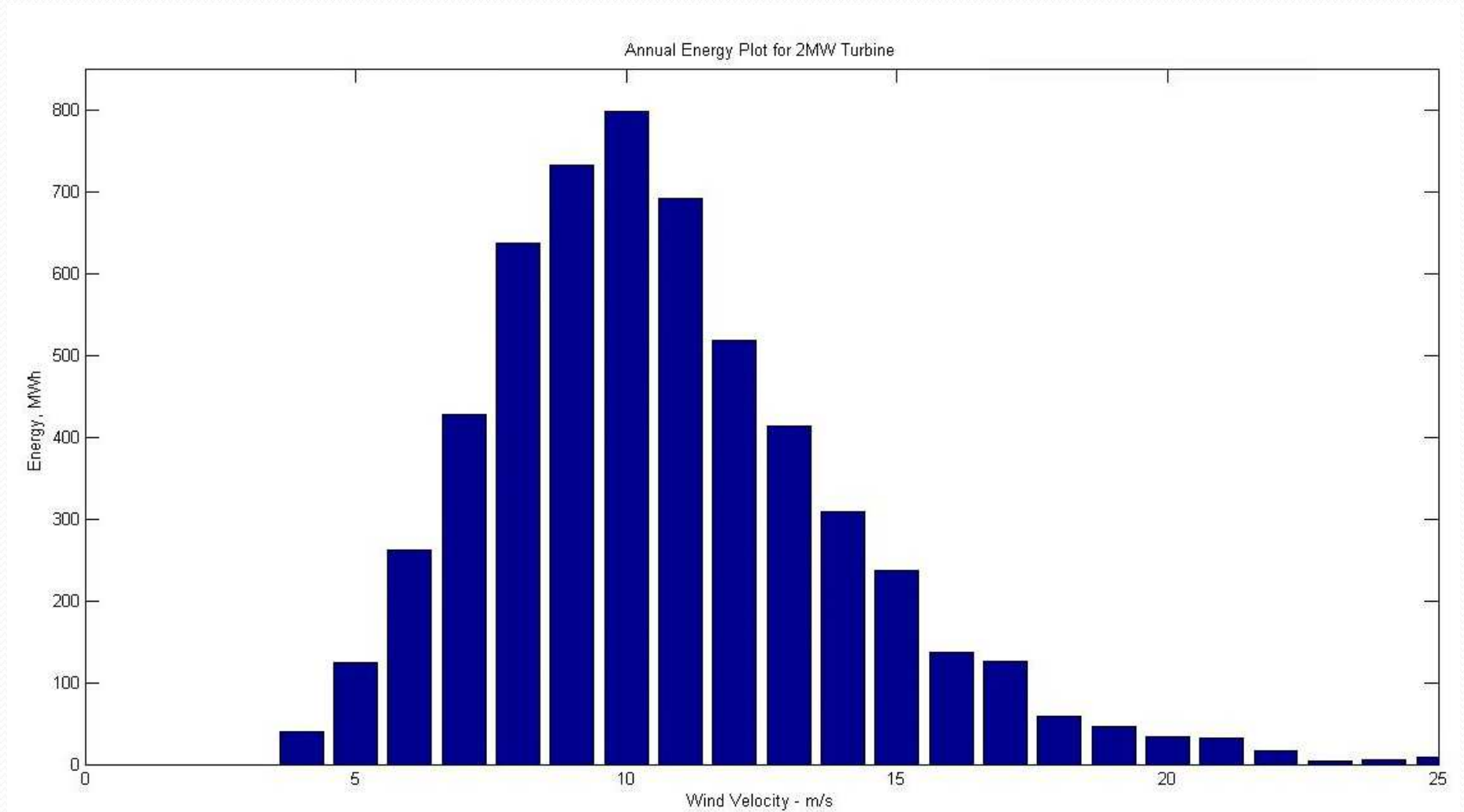
Figure 1 - Annual Energy Plot for 2MW Turbine
