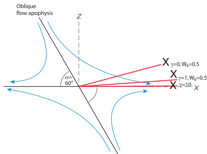
Figure SP2-8 Illustration of flow apophyses (blue lines) and the orientation of the finite strain ellipse ( X , red lines) for W_k = 0.5 and \gamma = 0, 1 , and 10 . The value for \gamma = 0 is the orientation of ISA_1 .
