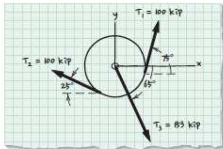
Free-body diagram
