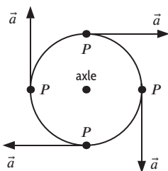
Figure 12.49: \vec{a} is the velocity of P relative to the axle
