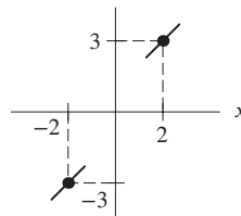
Figure 2.121: For f odd
