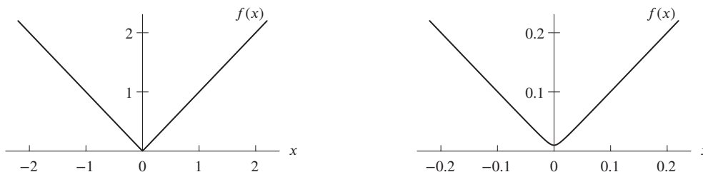
Figure 2.97: Close-ups of f(x) = (x^2 + 0.0001)^{1/2} showing differentiability at x = 0
