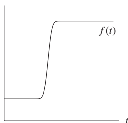
Figure 2.66: Step function
