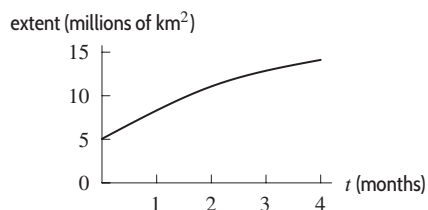
Figure 2.84: Arctic Sea ice extent from Oct. 1, 2018 to Feb. 1, 2019
