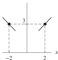
Figure 2.120: For f even
