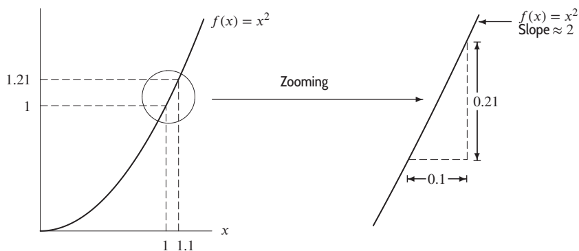
Figure 2.24: Graph of f(x) = x^2 near x = 1 has slope \approx 2
