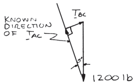
Force Triangle
