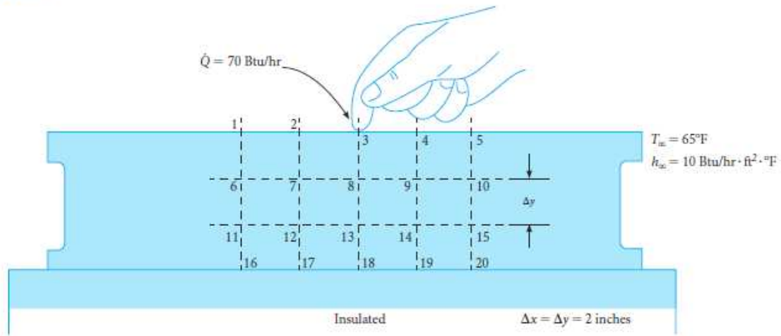
FIG 2-70 Surface plate.
