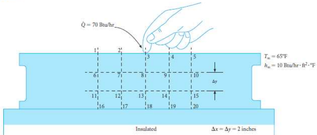
FIG 2-70 Surface plate.
