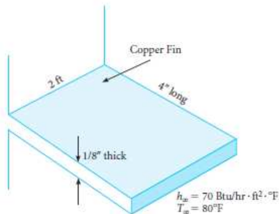
FIG 2-72 Problem 2-58.
