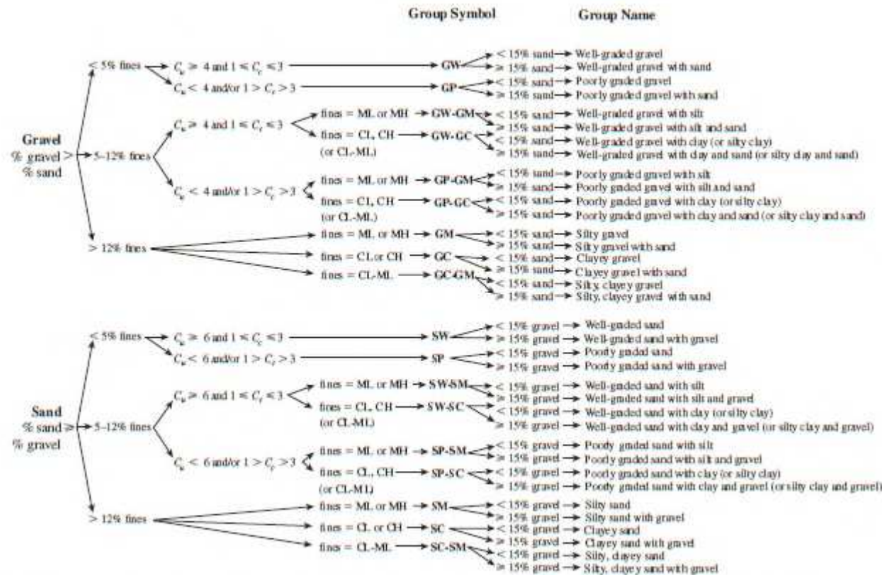
Figure 2.6 Flowchart for classifying coarse-grained soils (more than 50% retained on No. 200 Sieve) (After ASTM, 2011) (Based on ASTM D 2487-10: Standard Practice for Classification of Soils for Engineering Purposes (Unified Soil Classification)).
