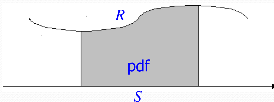
Continuous random variable
