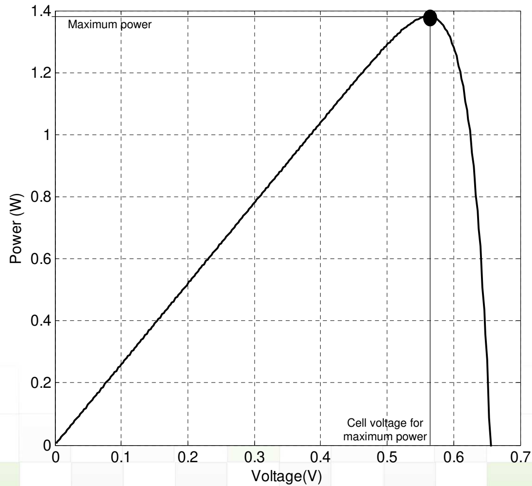
Figure 2.16 Power vs voltage characteristic
