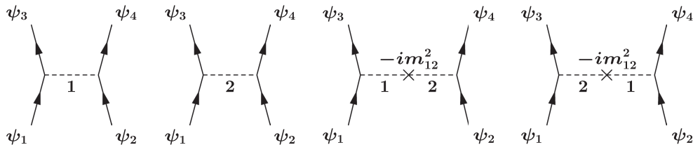
Figure 2.25 t -channel diagrams for \psi_1 \psi_2 \rightarrow \psi_3 \psi_4 , treating the m_{12}^2 term in (2.410) as a perturbative mass insertion. There are additional u channel diagrams with (3 \leftrightarrow 4) .
