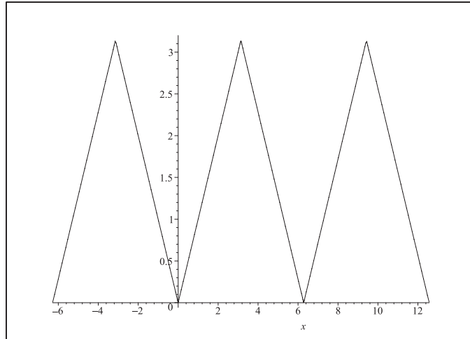
Figure 2.12: Plot of the first 10 terms of the Fourier series representation for f(x) = |x| on the interval x \in [-2\pi, 4\pi] .
